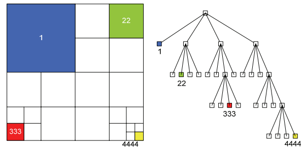
Figure 2. Multi-level image indexing by region quad-tree.
