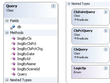
Figure 3. The query class diagram.
