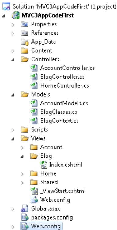
Figure 5: The new Blog Index View is added to the Views/Blog folder
