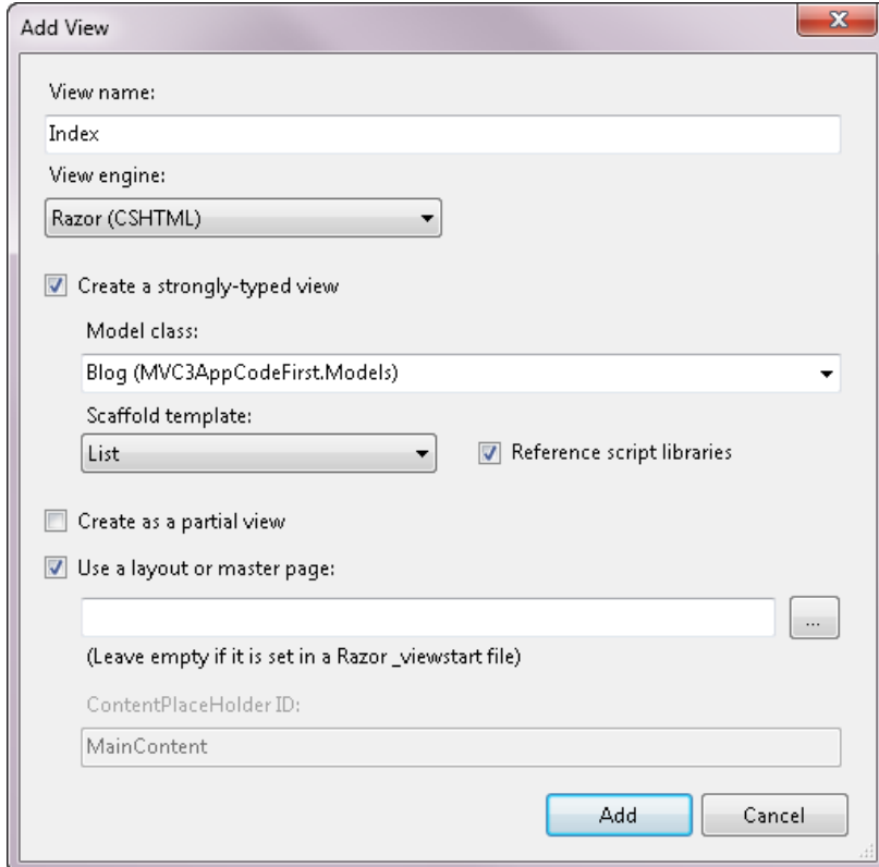
Figure 4: Creating a new view to display a list of Blog types
