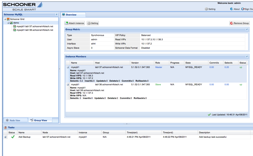
Figure 4: Schooner Active Cluster Synchronous Replication Administration GUI
