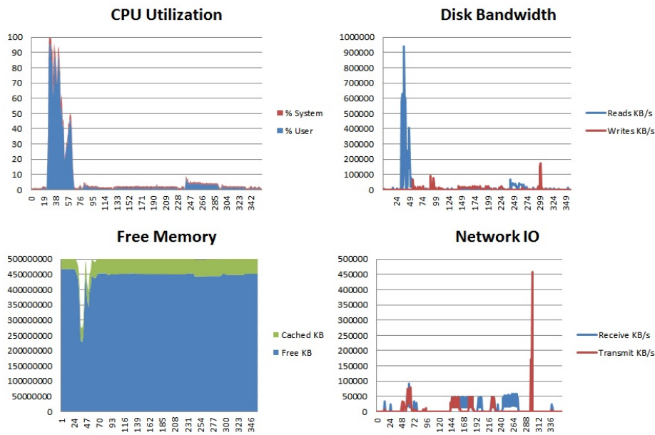
Fig. 3. System Utilization Statistics for Q1
